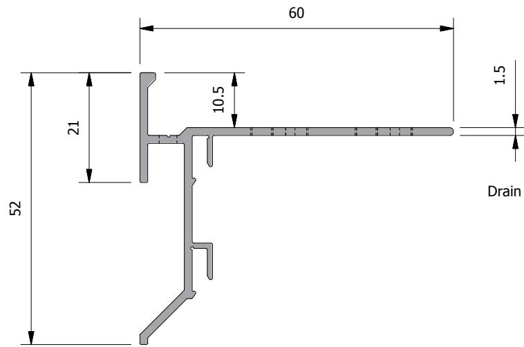
Sectional view
