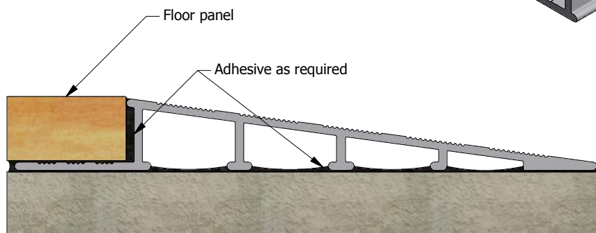
Typical installation detail
