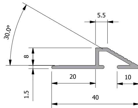
Sectional view
