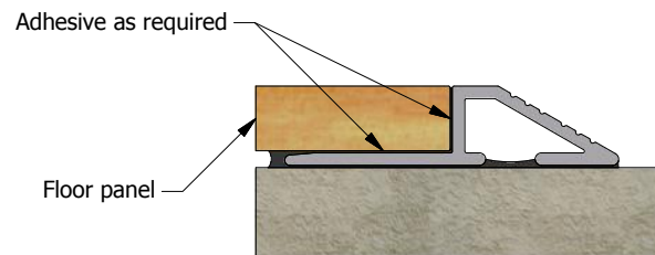
Typical installation detail
