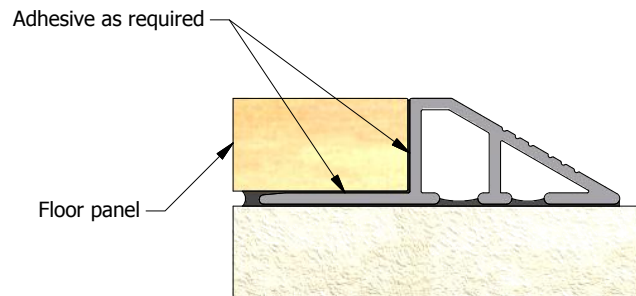
Sectional view
