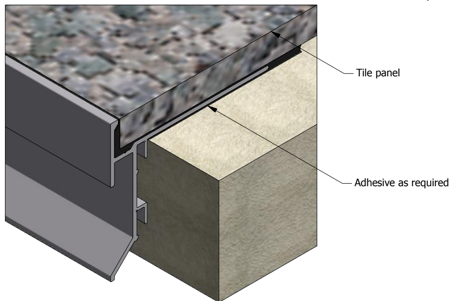
Typical installation detail
