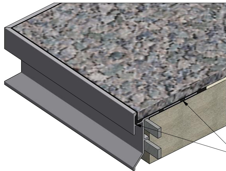
Typical installation detail
