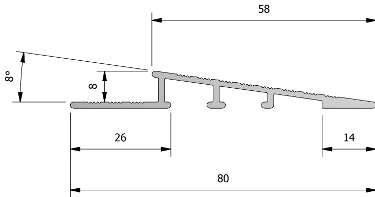
Sectional view
