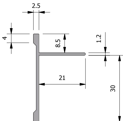
Sectional view
