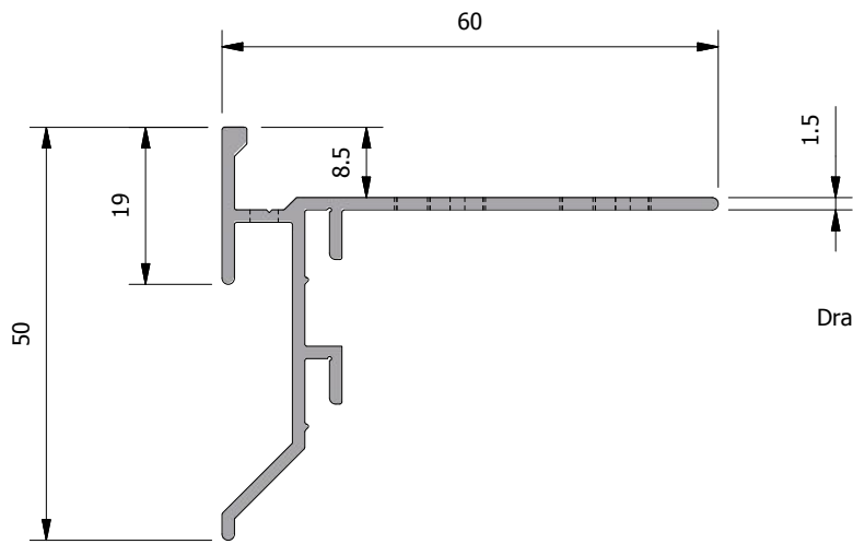
Sectional view
