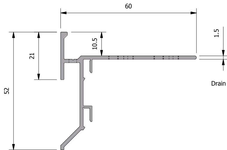
Sectional view
