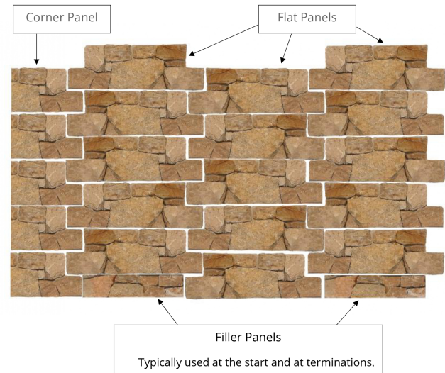
Typical Panel Configuration
